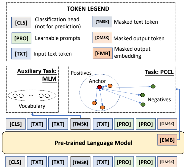
Figure 2: An overview of the CP-Tuning framework.
